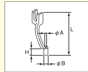
Intermediate presser
